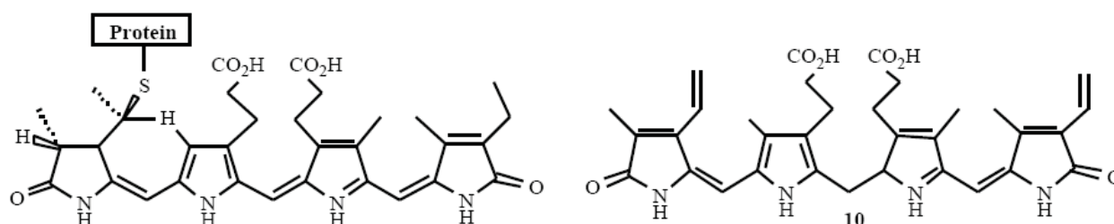
Chemical structure of phycocyanin bilin chromophore (open-chain tetrapyrrol) (a) and bilirubin (b). Adapted from Romay et. al
